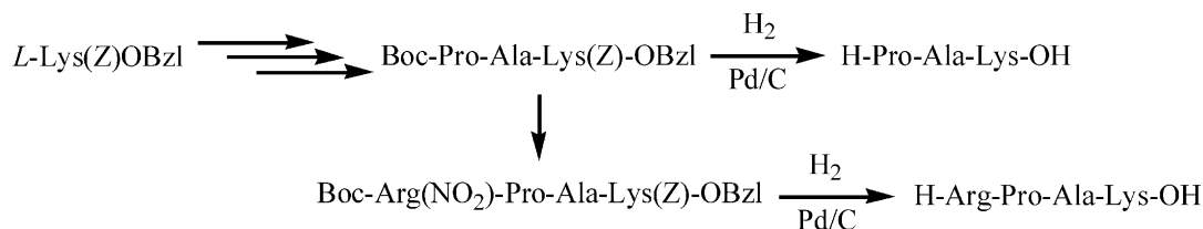
Scheme 3. Preparation of Arg-Pro-Ala-Lys-OH and Pro-Ala-Lys-OH. (1) General procedure for removal of Boc of the C-terminal component: The solution of 0.20 mmol of Boc protected compound in 2 mL of hydrogen chloride in ethyl acetate (4 mol/L) was stirred at room temperature for 3 h. (2) General procedure for coupling of C-terminal and N-terminal components: To a solution of 0.20 mmol of the N-terminal component in 5 mL of anhydrous THF at 0 °C 0.20 mmol of HOBt and 0.25 mmol of DCC were added. The reaction mixture was stirred at 0 °C for 24 h. To the solution 0.20 mmol of C-terminal component and 0.26 mmol of N -methylmorpholine were added. The reaction mixture was stirred at room temperature for 24 h.
